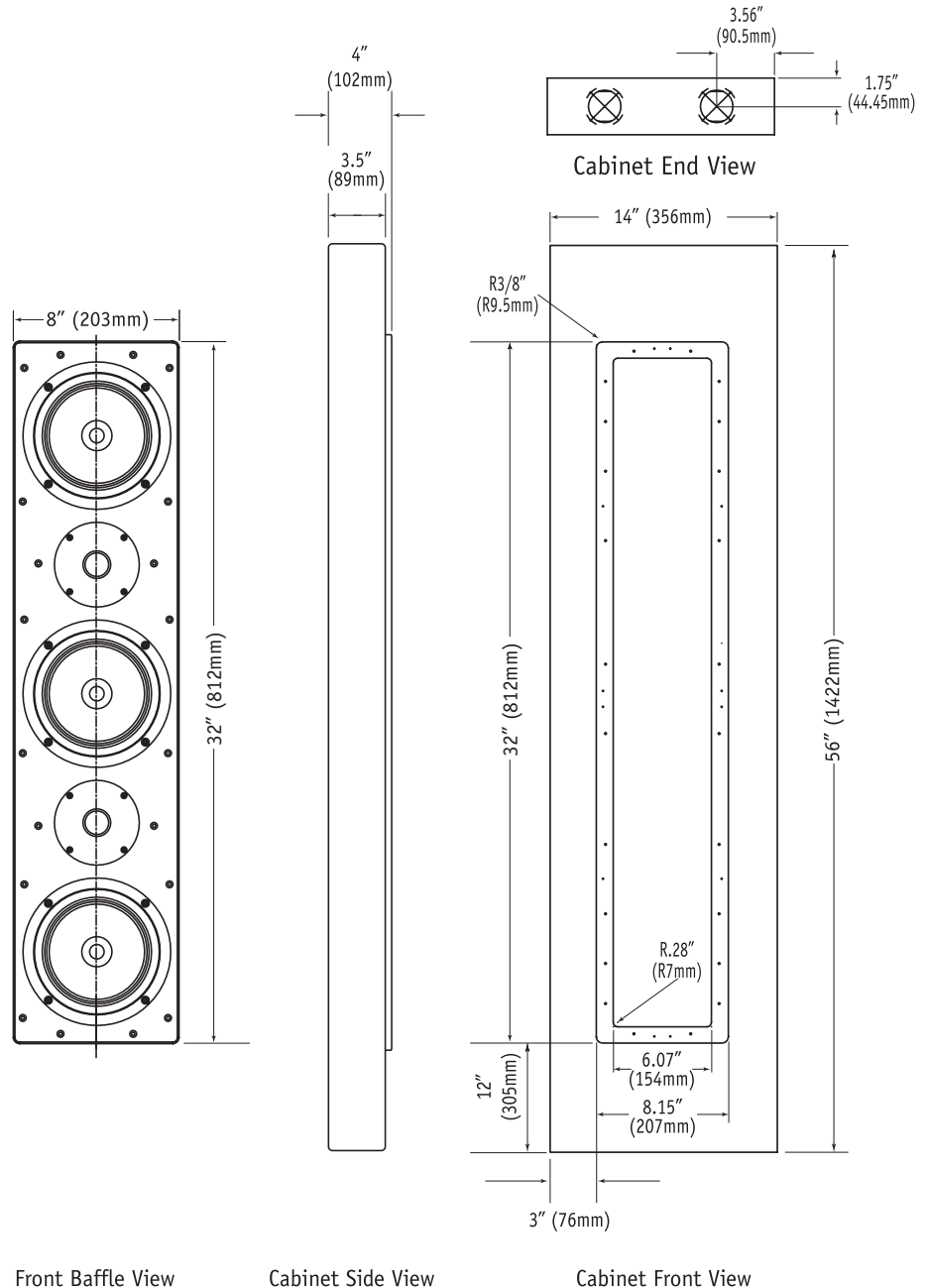
Front Baffle View
