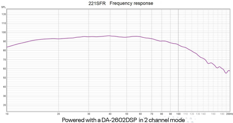
UNRIVALED 221 subwoofer includes calibrated RBH DA-2602DSP single or dual amps (4000W each)
